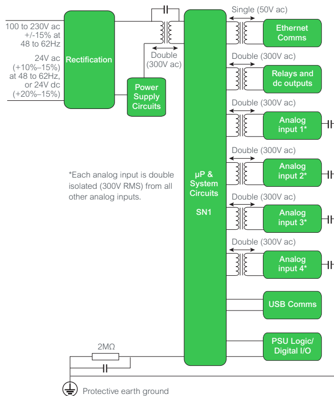
Isolation details
