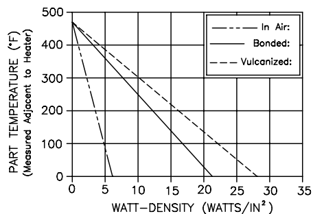
FIGURE 14: Maximum recommended watt-density for flexible rubber heaters vs. part (or ambient air) temperature for various mounting methods. For applications where watt-density may be higher consult factory.
